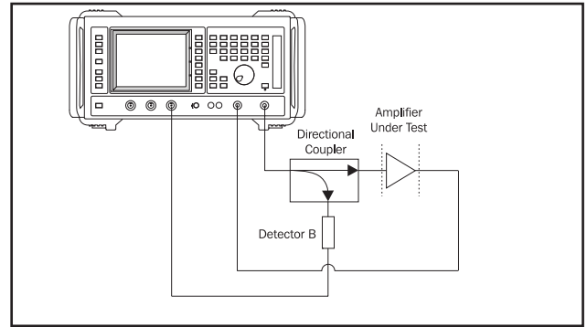
Figure 7 Gain Compression using the Tuned Input
