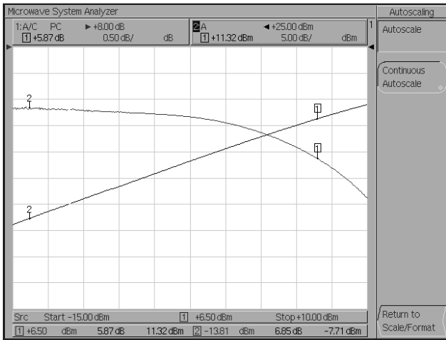
Figure 8 : Gain Compression Measured Using Setup in Figure 6
