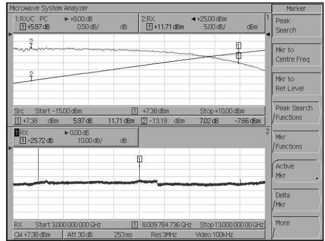
Figure 10 : Tuned Input Gain Compression with Output Spectrum at Compression
