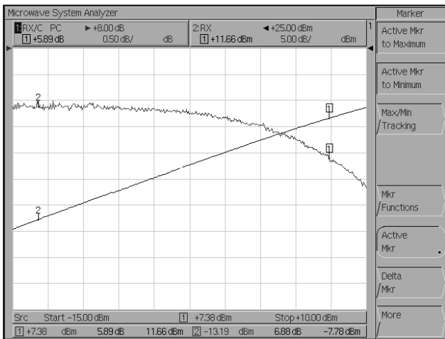
Figure 9 : Gain Compression Measured using Tuned Input
