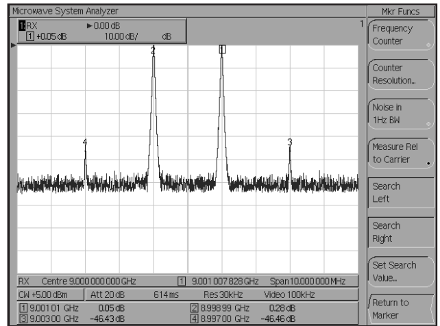
Figure 13 : Intermodulation Response
