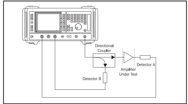
Figure 6: Gain compression Test System
