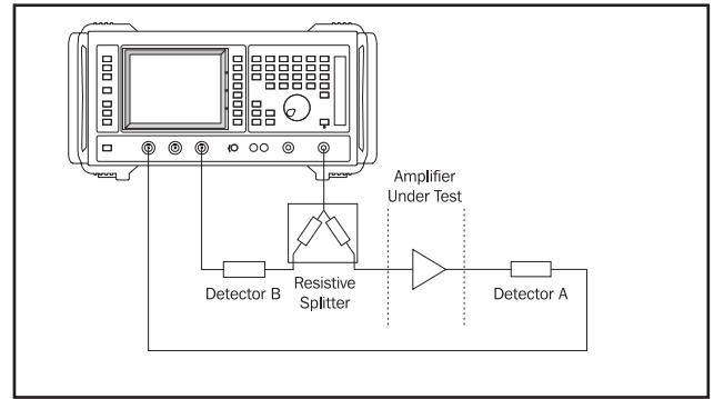
Figure 1 - Frequency response test system
