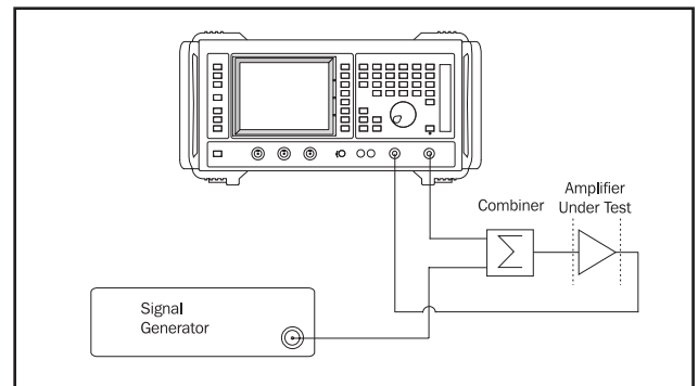
Figure 11 : Basic Intermodulation test setup
